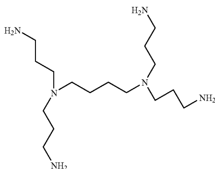
Polypropylenimine tetraamine dendrimer (DAB-AM-4: generation 1)
